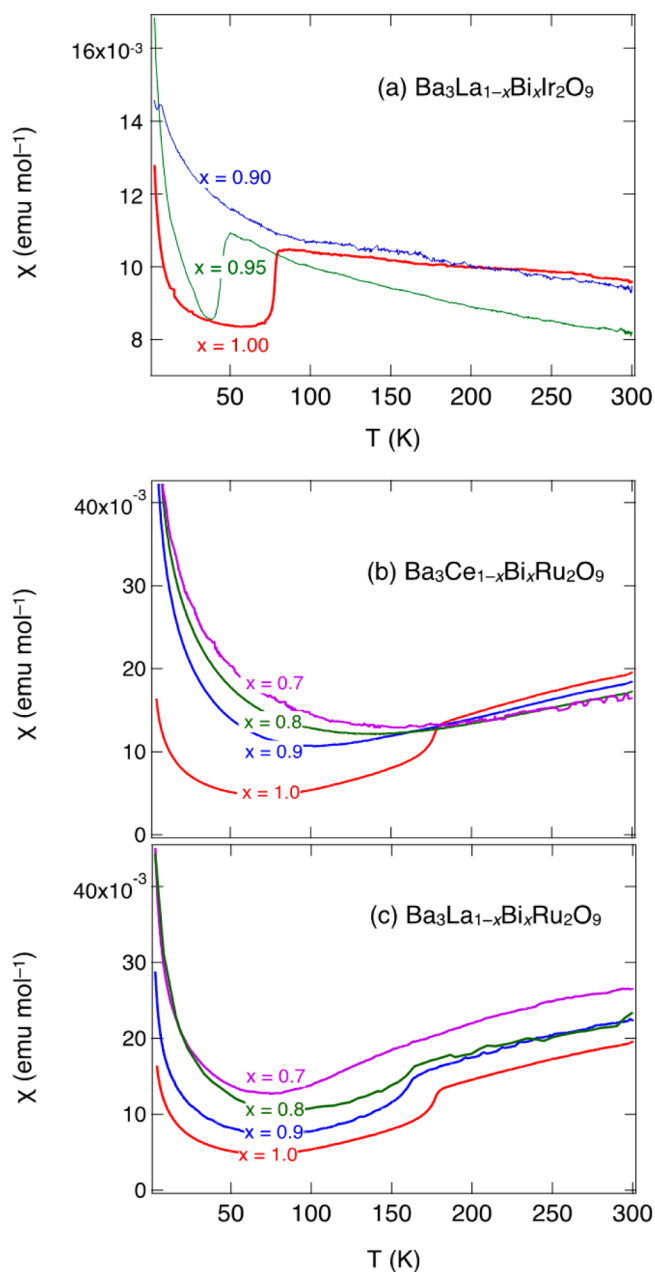
Figure 3. Magnetic susceptibility as a function of temperature for (a) \text{Ba}_3\text{La}_{1-x}\text{Bi}_x\text{Ir}_2\text{O}_9 , (b) \text{Ba}_3\text{La}_{1-x}\text{Bi}_x\text{Ru}_2\text{O}_9 , and (c) \text{Ba}_3\text{Ce}_{1-x}\text{Bi}_x\text{Ru}_2\text{O}_9 .
