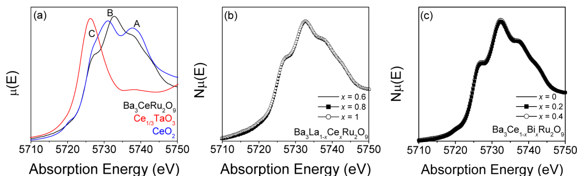
Figure 10. Representative normalized Ce L_{3} -edge XANES spectra of (a) Ce standards compared to \text{Ba}_3\text{CeRu}_2\text{O}_9 , (b) \text{Ba}_3\text{La}_{1-x}\text{Ce}_x\text{Ru}_2\text{O}_9 , and (c) \text{Ba}_3\text{Ce}_{1-x}\text{Bi}_x\text{Ru}_2\text{O}_9 . Spectra were collected for Ce-rich samples because of overlap with the Ba L_{2} -edge. All spectra were presented in fluorescence mode.
