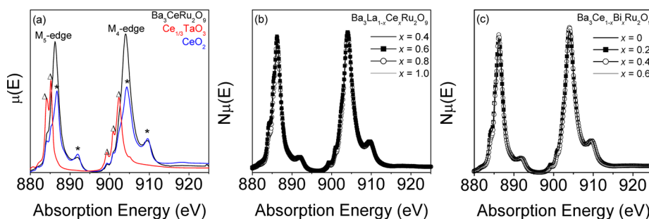
Figure 11. Representative normalized Ce M_{5,4} -edge XANES spectra of (a) Ce standards compared to \text{Ba}_3\text{CeRu}_2\text{O}_9 , (b) \text{Ba}_3\text{La}_{1-x}\text{Ce}_x\text{Ru}_2\text{O}_9 , and (c) \text{Ba}_3\text{Ce}_{1-x}\text{Bi}_x\text{Ru}_2\text{O}_9 . Peaks corresponding to \text{Ce}^{3+} and \text{Ce}^{4+} are marked as \Delta and * , respectively. All spectra were presented in TEY mode.
