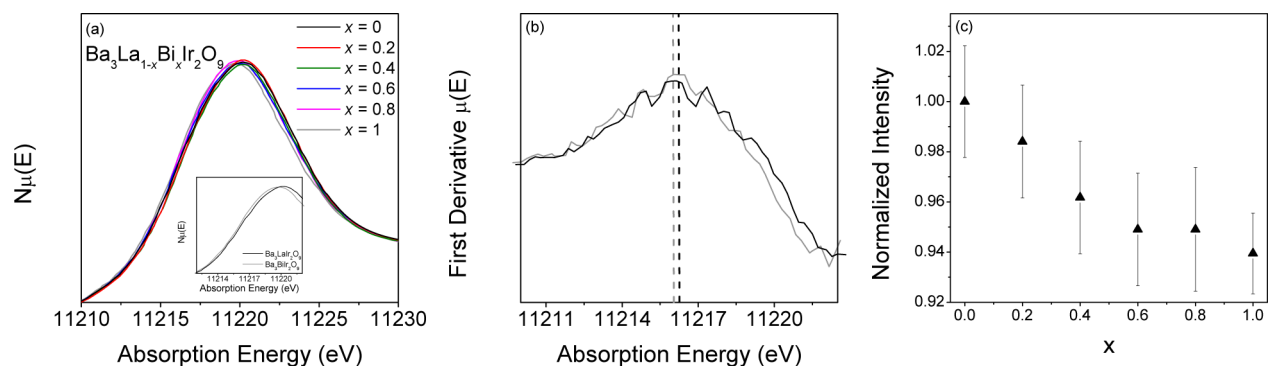
Figure 9. (a) Normalized Ir L_3 -edge XANES spectra of \text{Ba}_3\text{La}_{1-x}\text{Bi}_x\text{Ir}_2\text{O}_9 . Inset compares the edge onset for \text{Ba}_3\text{LaIr}_2\text{O}_9 and \text{Ba}_3\text{BiIr}_2\text{O}_9 . (b) The first derivative Ir L_3 -edge XANES spectra of \text{Ba}_3\text{LaIr}_2\text{O}_9 (black) and \text{Ba}_3\text{BiIr}_2\text{O}_9 . Dashed lines represent the Ir L_3 -edge absorption edge energies. (c) The Ir L_3 -edge integrated intensities, normalized to the integrated intensity of \text{Ba}_3\text{LaIr}_2\text{O}_9 . All spectra were presented in fluorescence mode.
