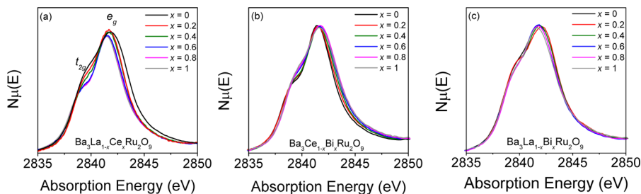
Figure 6. Representative normalized Ru L_3 -edge XANES spectra of (a) \text{Ba}_3\text{La}_{1-x}\text{Ce}_x\text{Ru}_2\text{O}_9 , (b) \text{Ba}_3\text{Ce}_{1-x}\text{Bi}_x\text{Ru}_2\text{O}_9 , and (c) \text{Ba}_3\text{La}_{1-x}\text{Bi}_x\text{Ru}_2\text{O}_9 . All spectra were presented in TEY mode.
