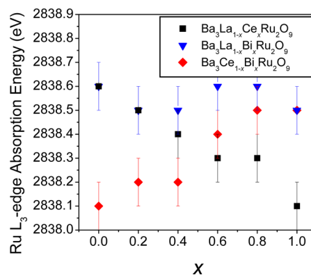
Figure 7. Plots of the Ru L_3 -edge absorption edge energy as a function of x for \text{Ba}_3\text{La}_{1-x}\text{Ce}_x\text{Ru}_2\text{O}_9 , \text{Ba}_3\text{Ce}_{1-x}\text{Bi}_x\text{Ru}_2\text{O}_9 , and \text{Ba}_3\text{La}_{1-x}\text{Bi}_x\text{Ru}_2\text{O}_9 .
