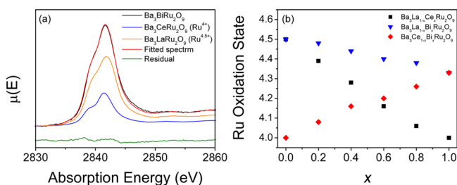
Figure 8. (a) Ru L_3 -edge XANES spectrum of \text{Ba}_3\text{BiRu}_2\text{O}_9 , including the corresponding fit and individual components ( \text{Ba}_3\text{LaRu}_2\text{O}_9 and \text{Ba}_3\text{CeRu}_2\text{O}_9 ). (b) Ru oxidation states as a function of x in \text{Ba}_3\text{La}_{1-x}\text{Ce}_x\text{Ru}_2\text{O}_9 , \text{Ba}_3\text{Ce}_{1-x}\text{Bi}_x\text{Ru}_2\text{O}_9 , and \text{Ba}_3\text{La}_{1-x}\text{Bi}_x\text{Ru}_2\text{O}_9 . All oxidation states were estimated from linear combination fitting analysis of the Ru L_3 -edge XANES spectra.
