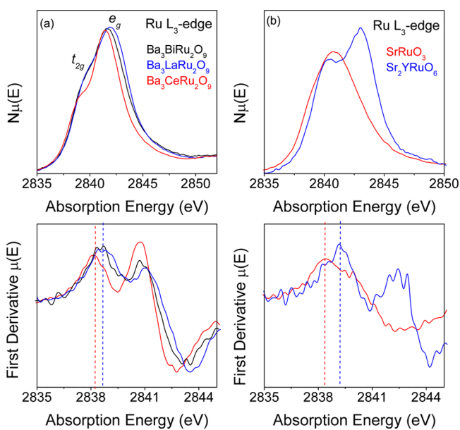
Figure 5. Normalized (upper) and first derivative (lower) Ru L_3 -edge XANES spectra of (a) \text{Ba}_3\text{BRu}_2\text{O}_9 ( B = \text{La}, \text{Ce}, \text{Bi} ) and (b) standards \text{SrRuO}_3 ( \text{Ru}^{4+} ) and \text{Sr}_2\text{YRuO}_6 ( \text{Ru}^{5+} ). All spectra were presented in TEY mode.
