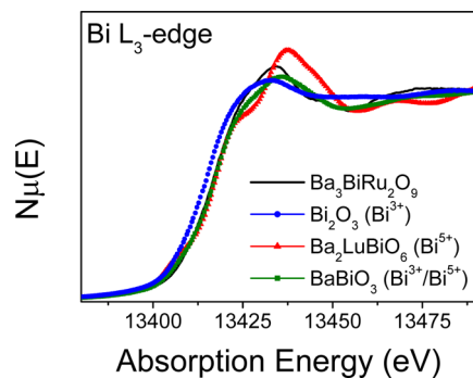
Figure 4. Normalized Bi L_3 -edge XANES spectra of \text{Ba}_3\text{BiRu}_2\text{O}_9 , \text{Bi}_2\text{O}_3 , \text{Ba}_2\text{LuBiO}_6 , and \text{BaBiO}_3 . All spectra were collected in fluorescence mode.
